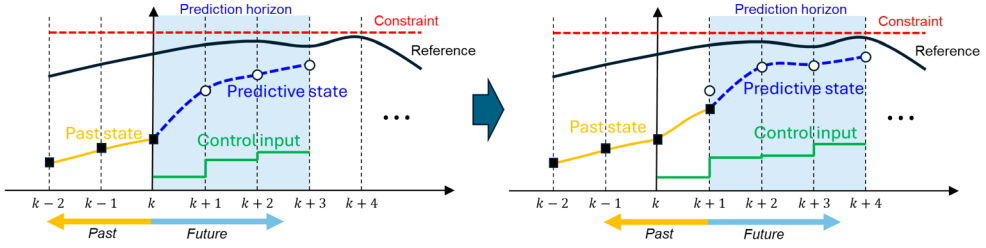
Figure 8. Illustration of model predictive control with moving prediction horizons.
